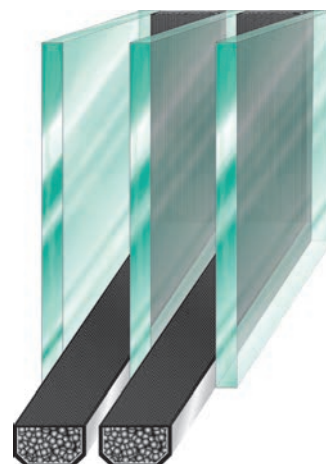
SANCO® ACS Randverbund
